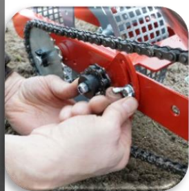
Chain tensioner with simple and super-fast tension-system
